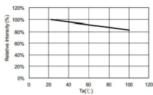
Fig.5- Relative Intensity (@100mA) vs. Ambient Temperature
