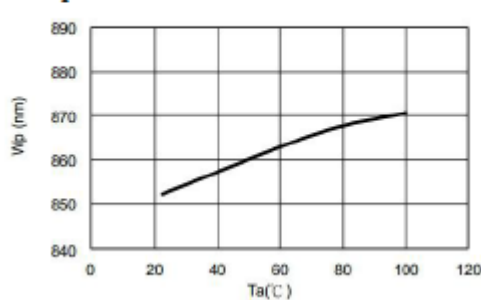
Fig.7- Peak Wavelength (@100mA) vs. Ambient Temperature.
