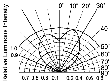
Radiation Pattern
