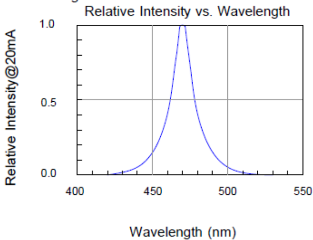
Fig.3 B CHIP
