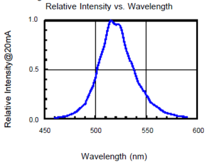
Fig.2 G CHIP
