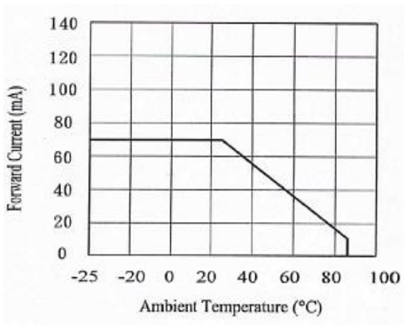
Fig 3. Forward Current vs. Ambient Temperature
