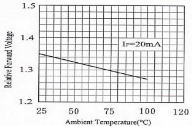
Fig.4 Forward Voltage vs. Ambient Temperature(°C)
