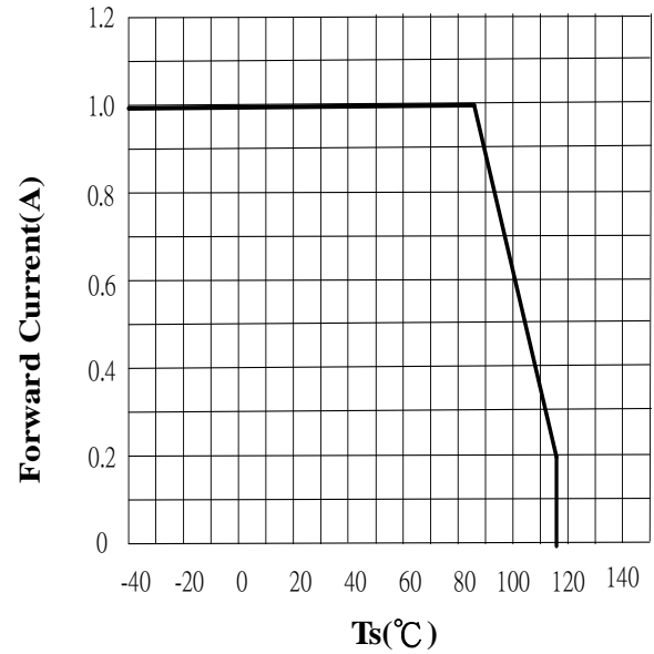
Forward Current & Ambient Temperature
