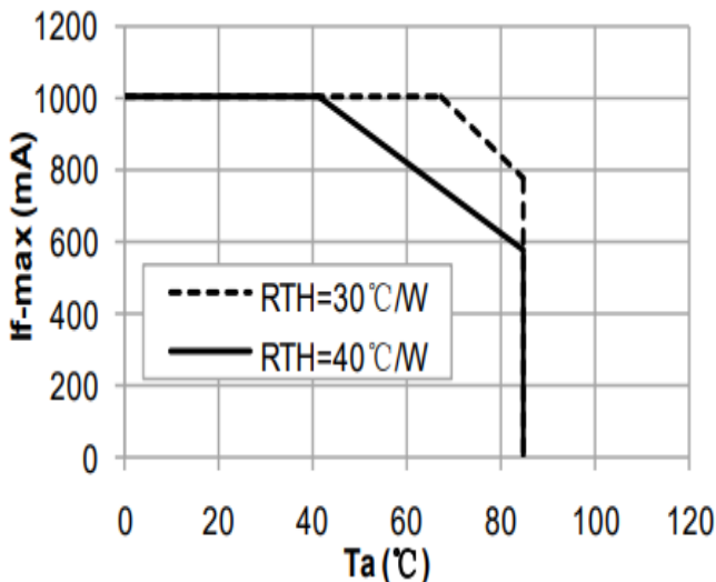
Maximum Driving Forward DC Current vs. Ambient Temperature ( Derating based on Tj max=145°C)
