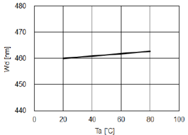
Dominant Wavelength (@700mA) vs. Ambient Temperature
