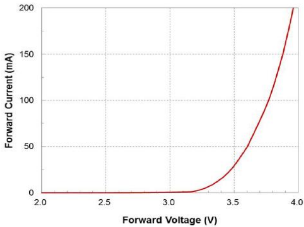
Current vs. Voltage
