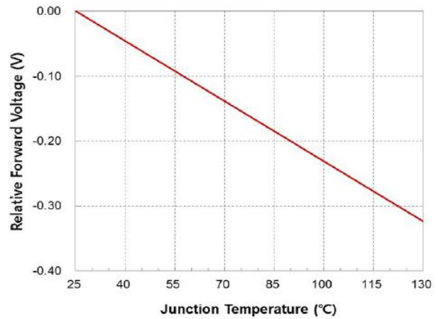
Forward Voltage Shift vs. Tj
