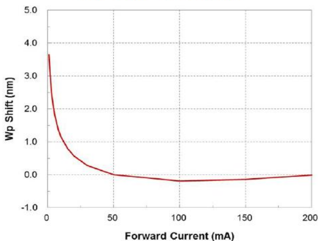
Wp Shift vs. Current
