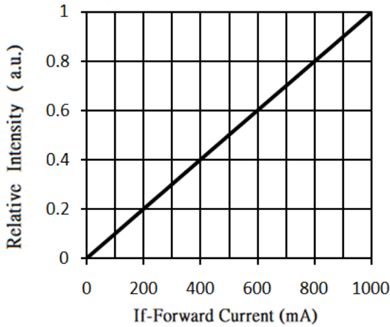
Fig.1-Relative Intensity VS. Forward Current
