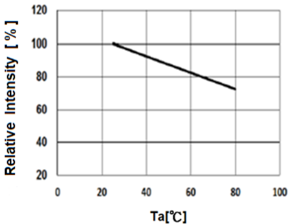
Fig.3-Relative Intensity vs.Ambient Temperature
