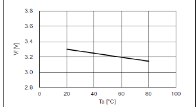
Fig.4 – Forward Voltage (@350mA) vs. Ambient Temperature
