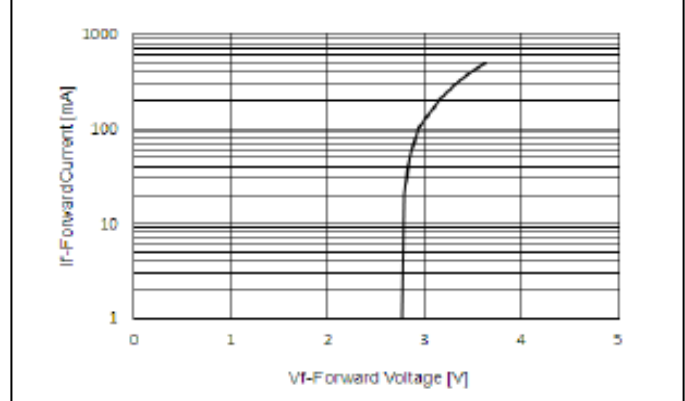
Fig.2 – Forward Current vs. Forward Voltage
