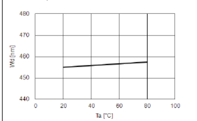
Fig.5 – Dominant Wavelength (@350mA) vs. Ambient Temperature
