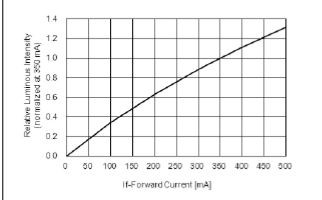
Fig.1 – Relative luminous Intensity vs. Forward Current
