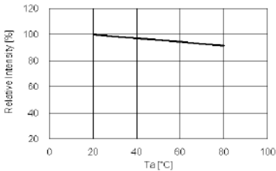
Fig.3 – Relative Intensity (@350mA) vs. Ambient Temperature
